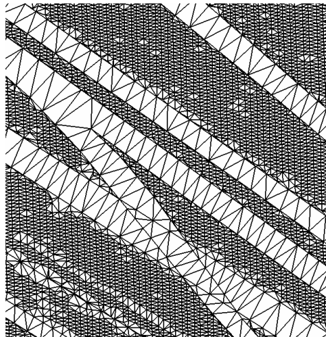
Figure 1 Constrained TIN model with roads and grass land.
