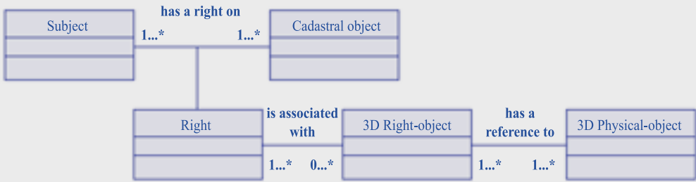
Figure 8: UML class diagram of 3D right-objects.
