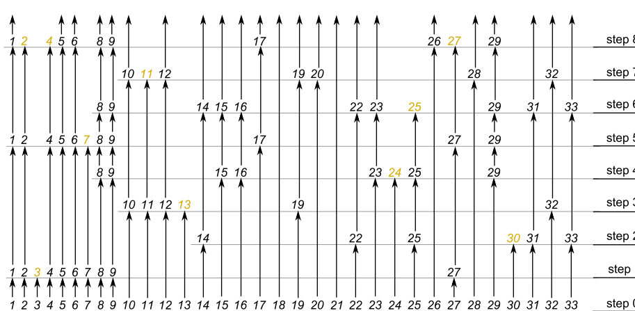
Fig. 9. Edge hierarchy for generalisation process of Fig. 6.
