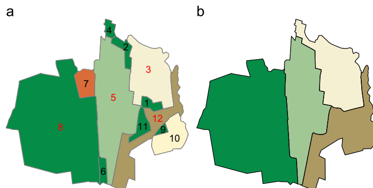
Fig. 5. Samples from two datasets that together can be used as input for Algorithm 1: detailed dataset (a) can be transformed into generalised dataset (b) applying merge operations only. Areas of detailed dataset are labelled with their IDs, region centres are shown by red labels. (For interpretation of the references to colour in this figure legend, the reader is referred to the web version of this article.)
