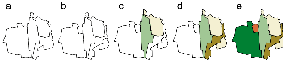
Fig. 12. Visualising sample data at scale 1:125 000 (iteration 6) on importance order: (a) valid edges of imp\_high > 8 ; (b) valid edges of imp\_high > 6 ; (c)–(e) valid areas of imp\_high greater than 8–6, respectively. Edges are drawn first in the importance order; when all edges are received areas are built and visualised based on class information.
