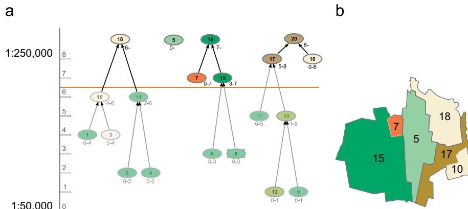
Fig. 10. Reconstructing a representation of certain LoD by selection in face hierarchy: (a) selecting areas in face hierarchy for scale 1:125 000, corresponding to iteration 6; (b) valid areas at iteration 6. These are leaf nodes after cutting face hierarchy at level 6.
