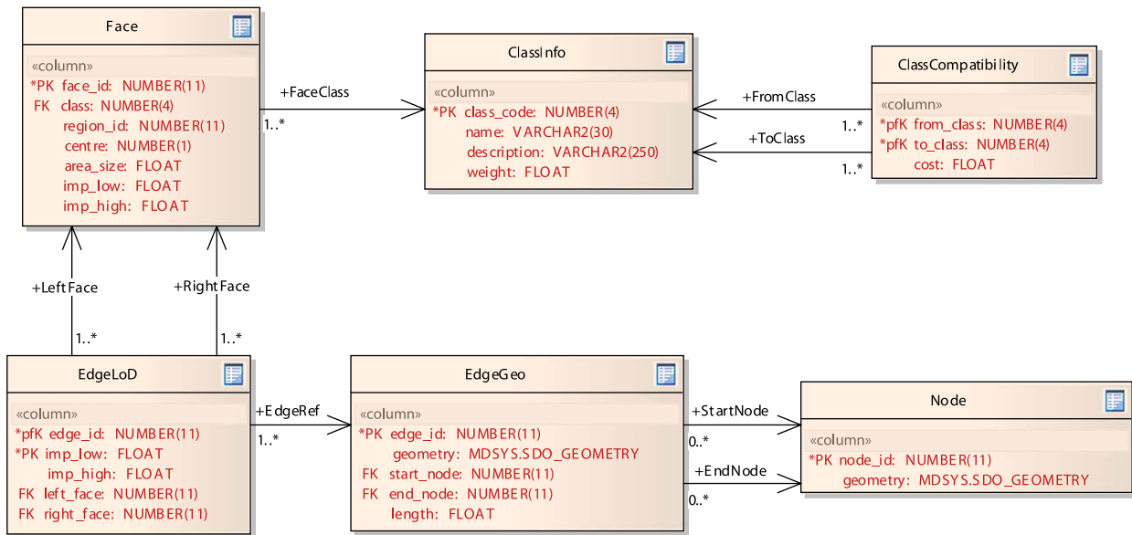
Fig. 11. UML diagram of tables and relationships that store constrained tGAP information in Oracle Spatial. PK shows a primary key, FK shows a foreign key, and pK shows a foreign key that is part of a primary key.
