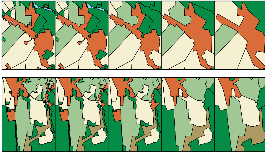
Fig. 7. Two examples processed with Algorithm 1. From left to right: most detailed dataset with additional boundaries S_{overlay} , found intermediate representations, and dataset generalised by optimisation S_{lowLoD} .
