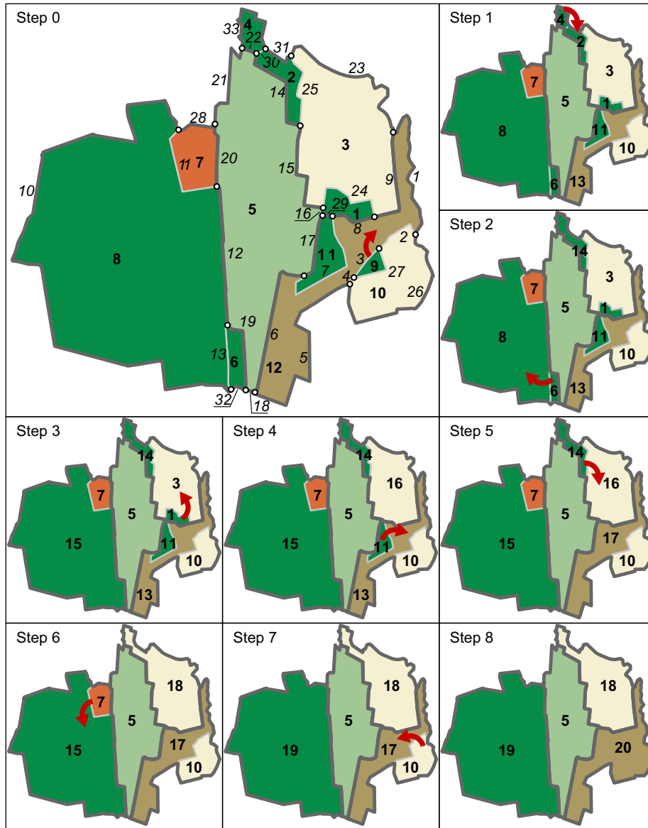
Fig. 6. Steps of iterative generalisation with Algorithm 1 for datasets of Fig. 5. Areas are labelled with their Ids, Ids of boundary lines are given for step 0.
