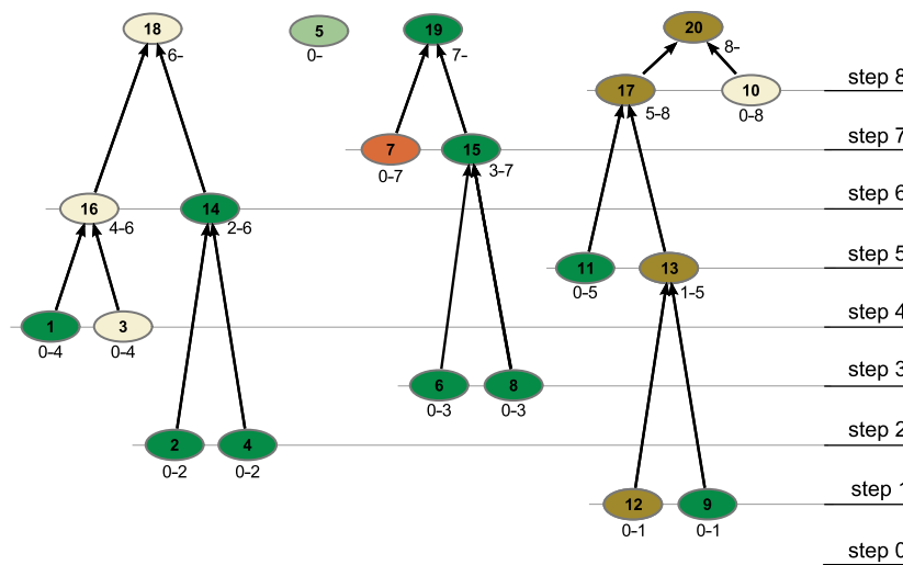
Fig. 8. Face hierarchy for generalisation process of Fig. 6. Each node corresponds to an area; labels show area Ids and validity ranges (below). Arrows depict merging of two areas into parent area.
