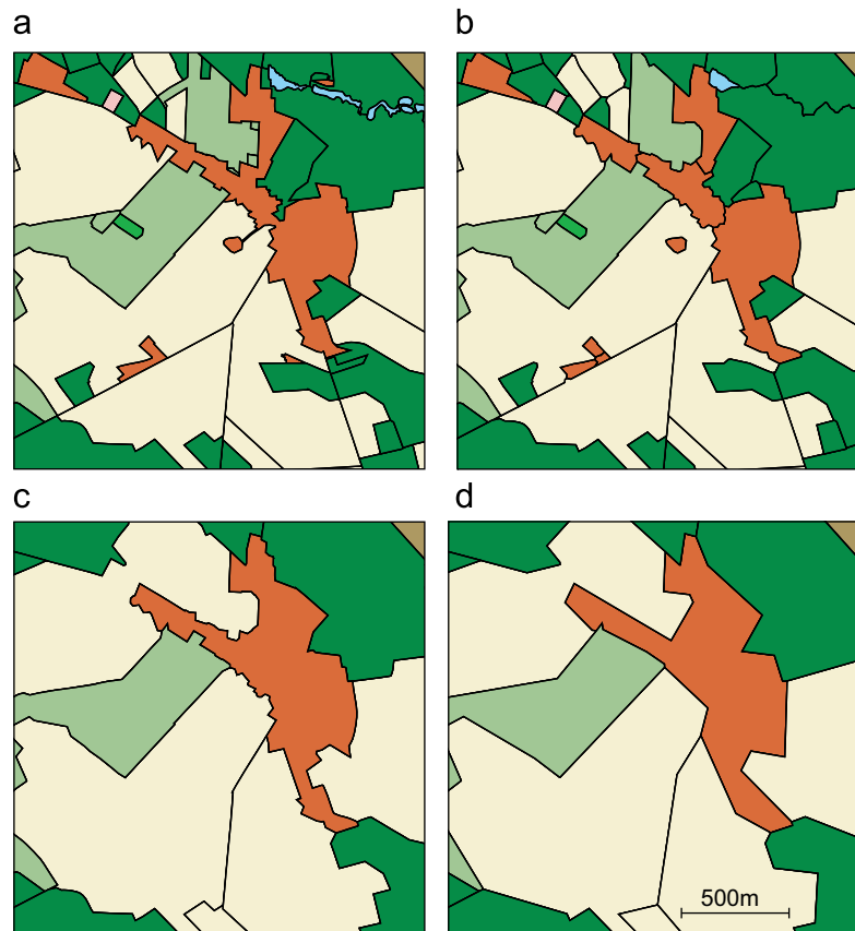
Fig. 3. Applied generalisation workflow. (a) Original dataset S_{\text{highLoD}} ; (b) result of collapse by skeletons S_{\text{coll}} ; (c) result of aggregation S_{\text{aggr}} ; (d) result of line simplification S_{\text{lowLoD}} .
