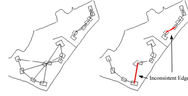
Figure 4: Initial graph, its derived MST and inconsistent edges
