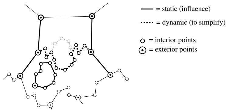
Fig. 3. Dynamic polylines will be simplified (only one in this Figure), static polylines can have an influence on the simplification. Note that the alternative is illustrated, in which only the polylines that are incident to a merge boundary will be simplified.
