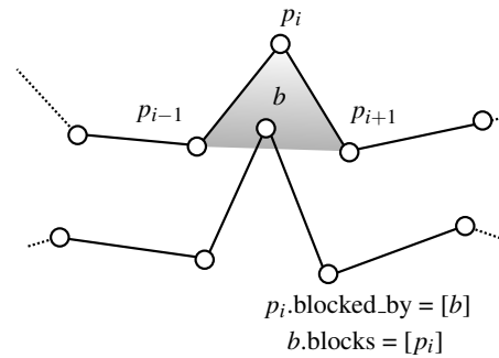
Fig. 4. As b blocks the removal of p_i , the blocks and blocked by lists are filled accordingly.
