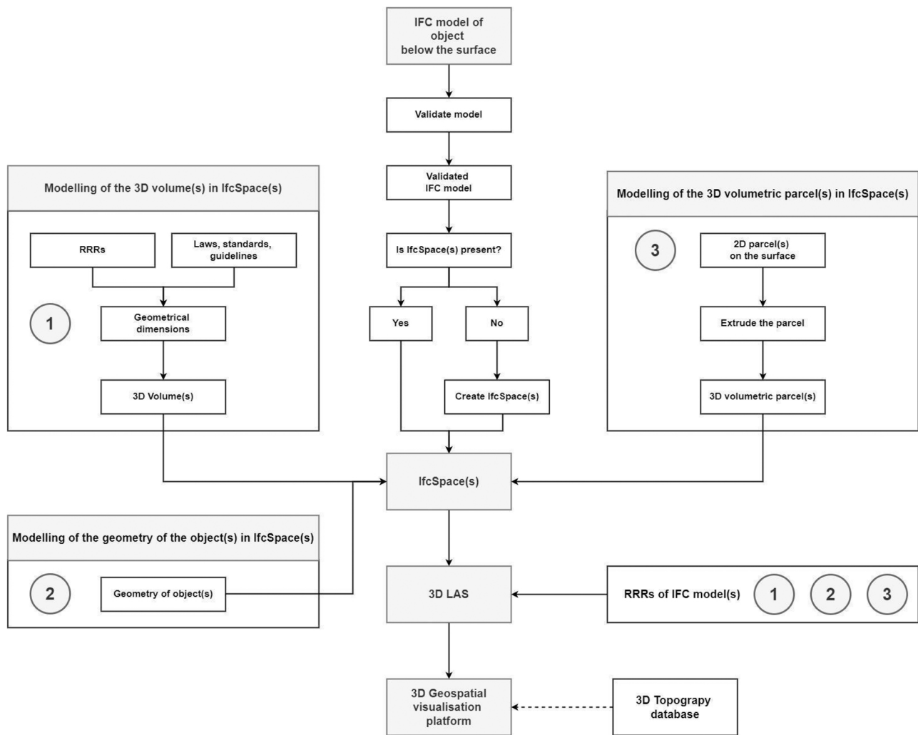
Fig. 6. Technical workflow.
