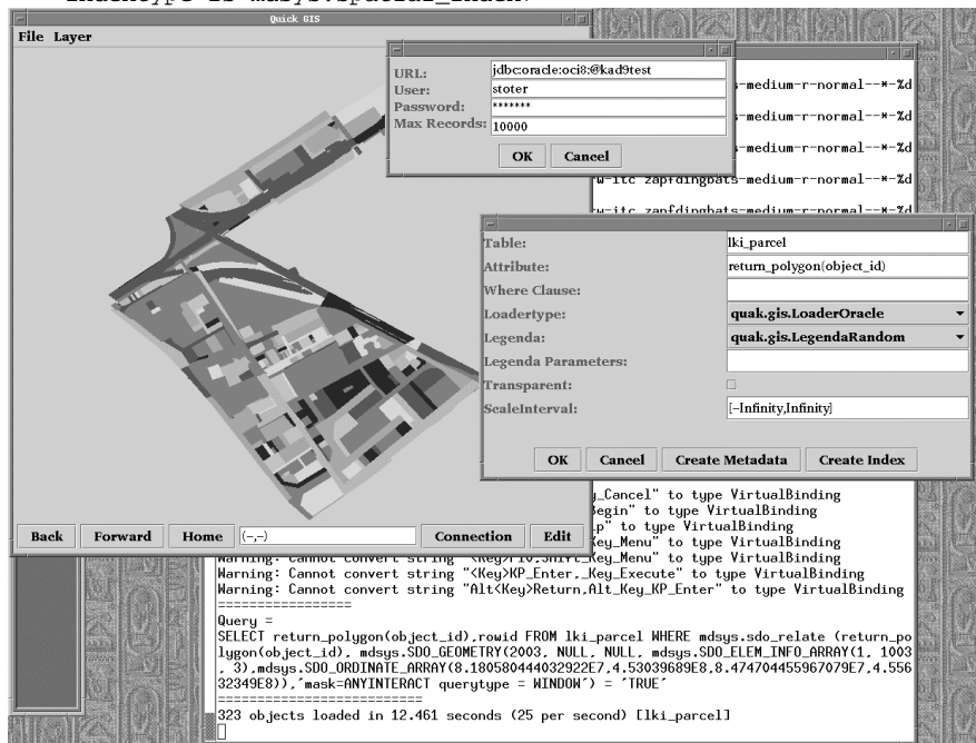
Figure 2: Viewing topological data in a viewer that is not topology aware
