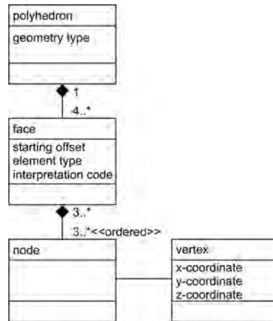
Figure 7.11: UML class diagram describing storage of polyhedron primitive.
