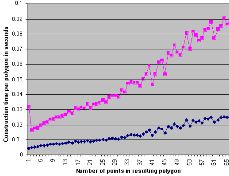
Figure 7.6: Construction time per polygon for different number of points in the resulting polygon. The black line represents the implementation based on the relationships between edges and the grey line represents the left-right implementation.
