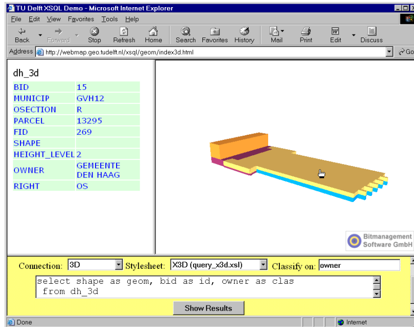
Figure 8.9: Screen dump of second prototype (based on XSQL and X3D).
