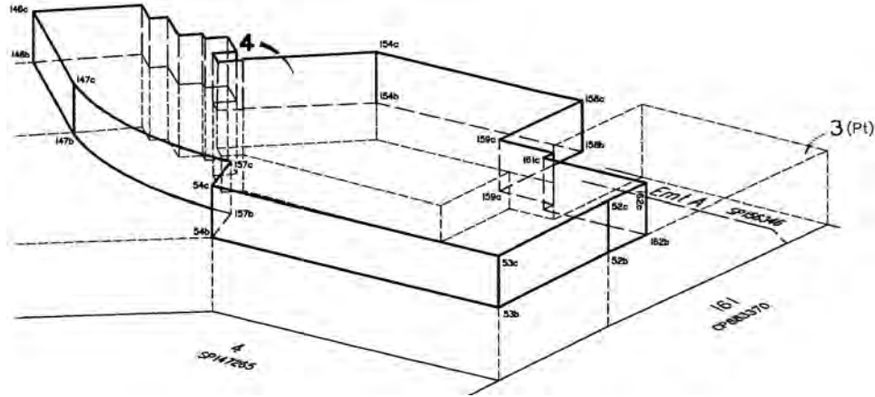
Figure 12.12: Volumetric parcel defined with more complex geometry than polyhedron.
