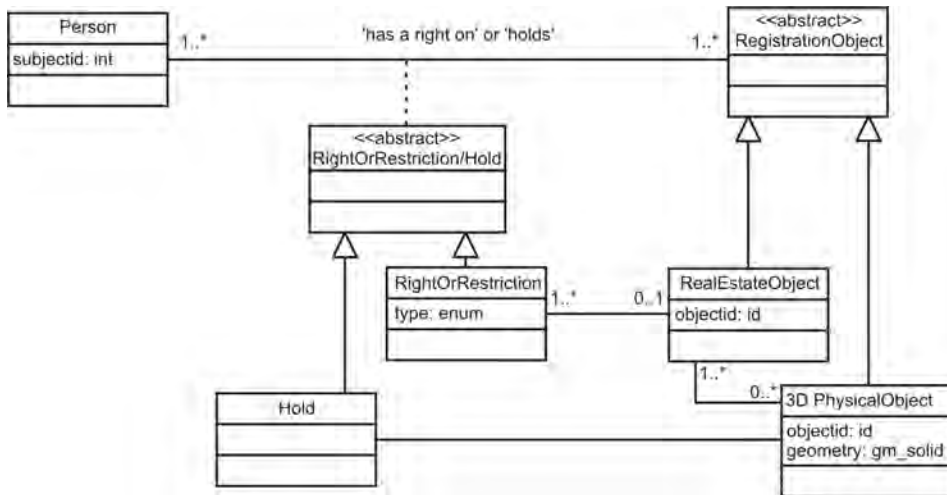
Figure 10.5: UML class diagram of 3D physical objects.
