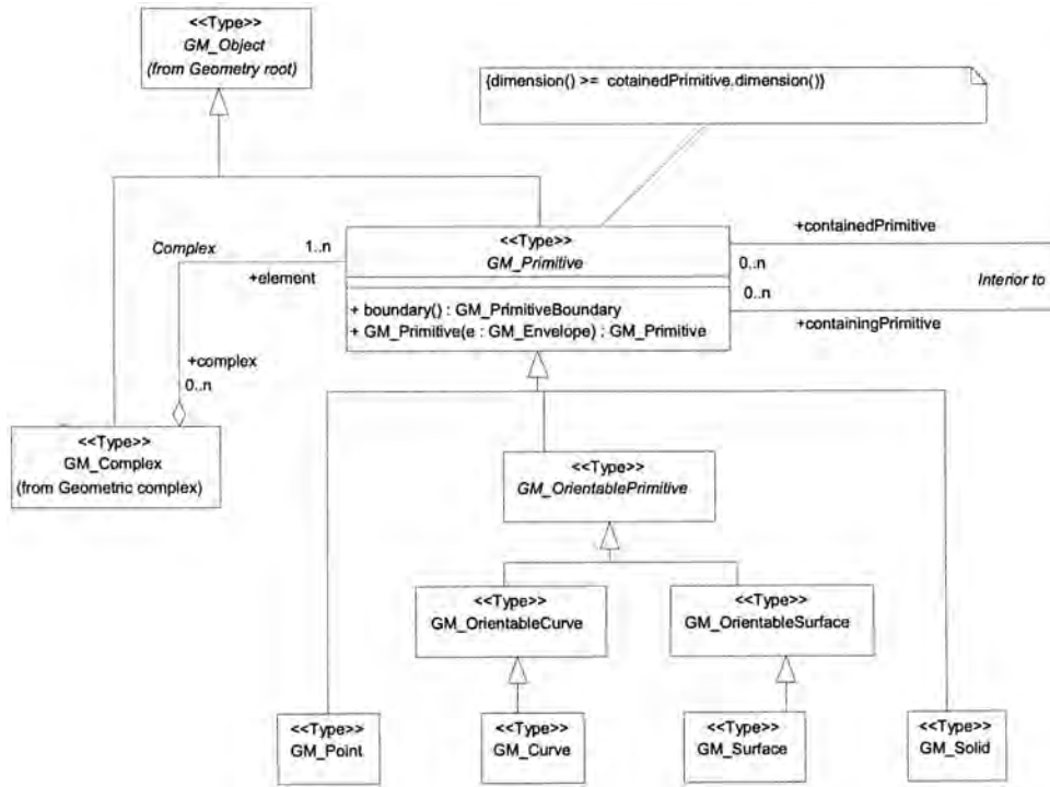
Figure 10.4: UML class diagram of gm-primitive as defined by OGC and ISO, taken from [152].
