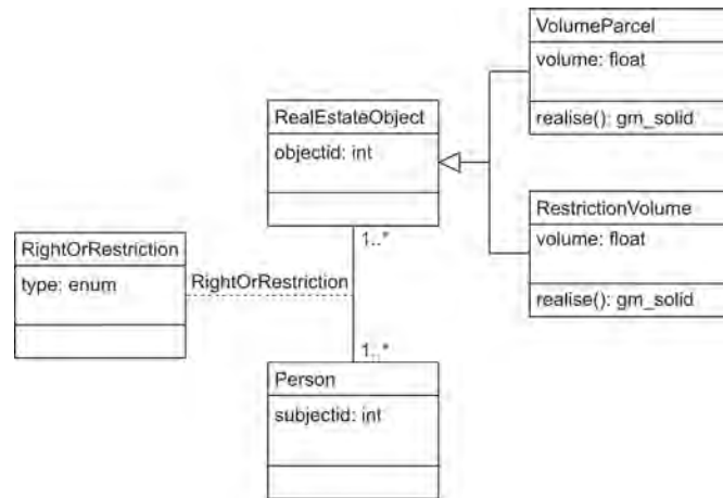
Figure 10.7: UML class diagram of a full 3D cadastre that only supports volume parcels. The volume parcels are part of a space partition.
