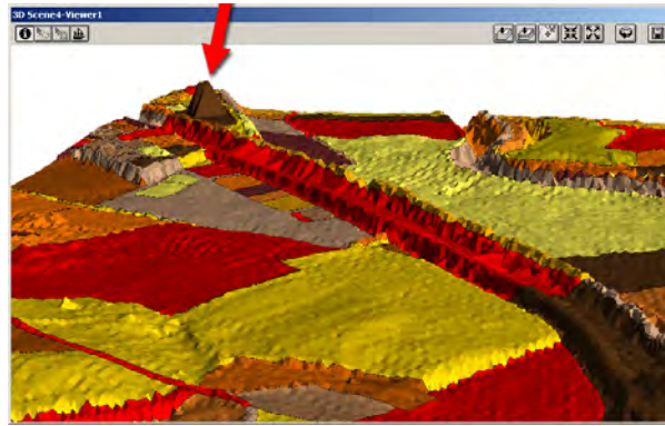
Figure 9.8: Conforming TIN in which point heights and 2D planar partition of parcels are integrated.
