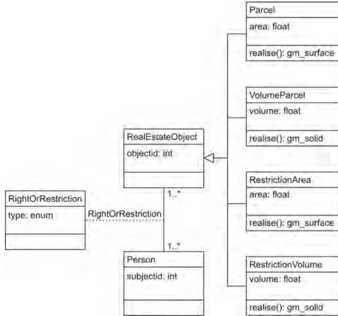
Figure 10.6: UML class diagram of full 3D cadastre that supports both infinite parcel columns and volume parcels. The parcel objects are part of a 2.5D partition.
