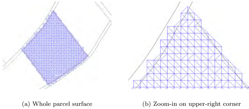
Figure 9.5: A parcel surface extracted from the DBMS based on an unconstrained TIN.
