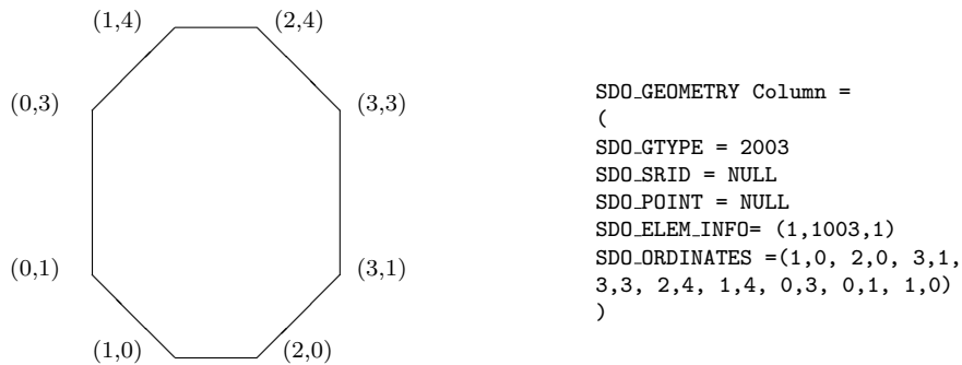
Figure 7.1: Example of storing a polygon using Oracle's spatial data type.
