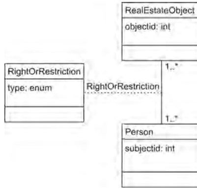
Figure 2.2: The current administrative cadastral data model in a UML class diagram.
