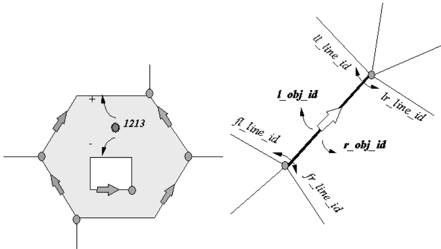
Figure 7.3: Topological structure in the spatial DBMS of the Netherlands' Kadaster, taken from [136].
