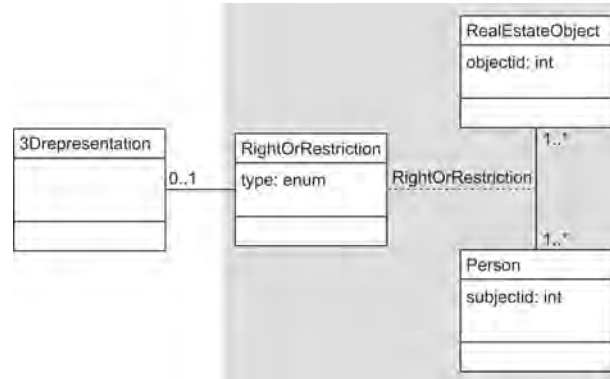
Figure 10.1: UML class diagram of the hybrid cadastre. The 3D representation refers to either a volume to which a person is entitled or a physical object.
