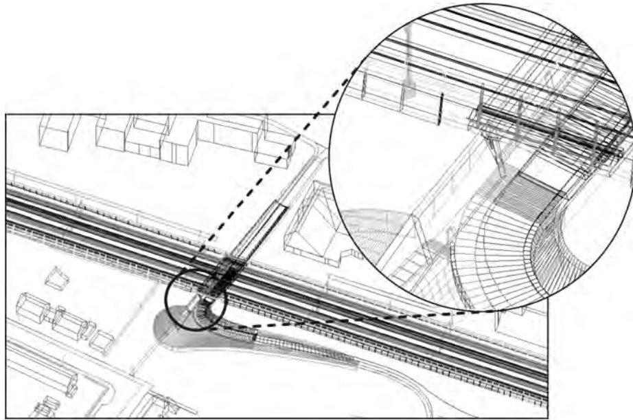
Figure 11.2: The CAD model designed for a cycle tunnel in Houten, the Netherlands (by courtesy of Holland Railconsult).
