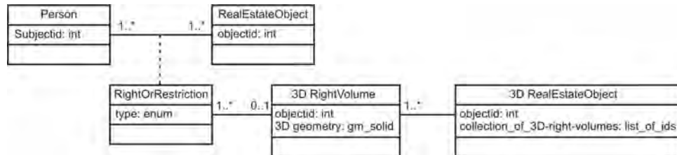
Figure 10.3: UML class diagram of 3D right-volumes.
