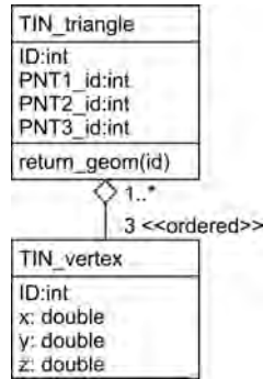
Figure 9.4: UML class diagram of TIN data structure.
