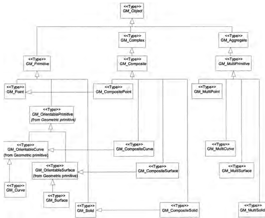
Figure 6.4: UML class diagram of geometry basic classes with specialisation relations, taken from [152].
