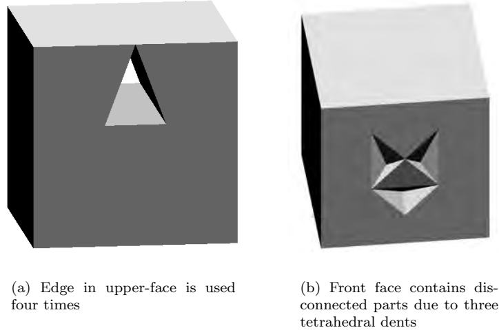
Figure 7.14: Valid polyhedra which are determined as invalid by the implementation.
