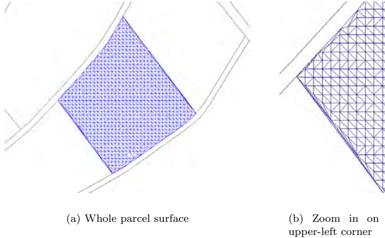
Figure 9.6: A parcel surface based on a constrained TIN.
