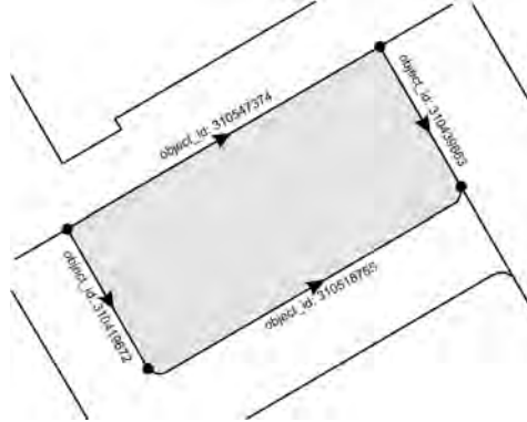
Figure 7.5: Id's and direction of boundaries of parcel 603.
