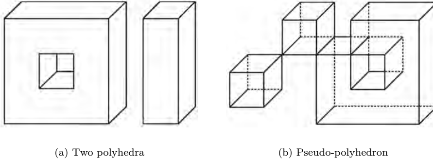
Figure 7.12: Examples of polyhedra.
