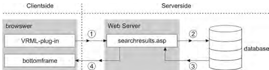
Figure 8.7: Model of the architecture of the prototype.
