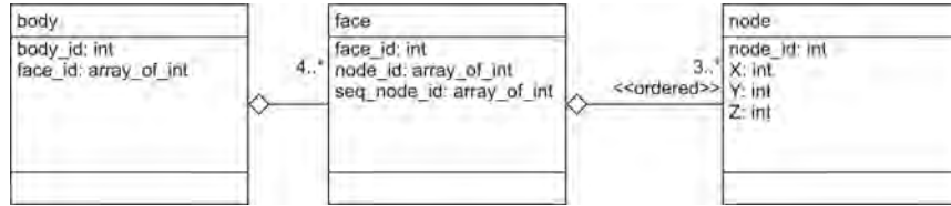
Figure 7.9: UML class diagram of Simplified Spatial Model [240].
