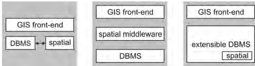
Figure 6.3: Evolving architectures of GIS. Left: dual architecture; middle: layered architecture, right: integrated architecture, taken from [221].
