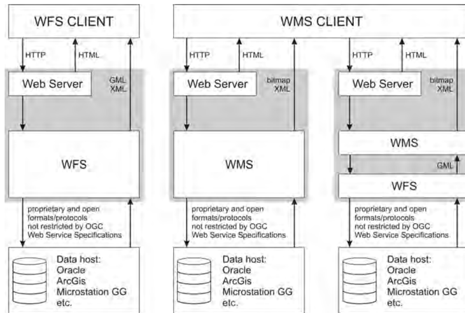
Figure 6.5: System architecture for disseminating geo-information using Web Map and Web Feature Services.
