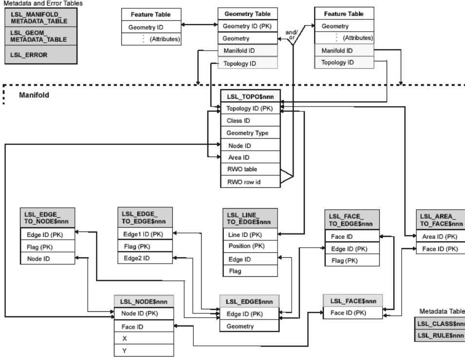
Figure 7.8: Radius Topology database tables (version 1.0), taken from [98].
