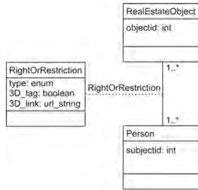
Figure 10.2: UML class diagram of 2D cadastre with tags to 3D situations.
