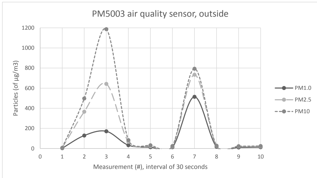
Figure 4: Extra tests with PMS5003 air quality sensor
