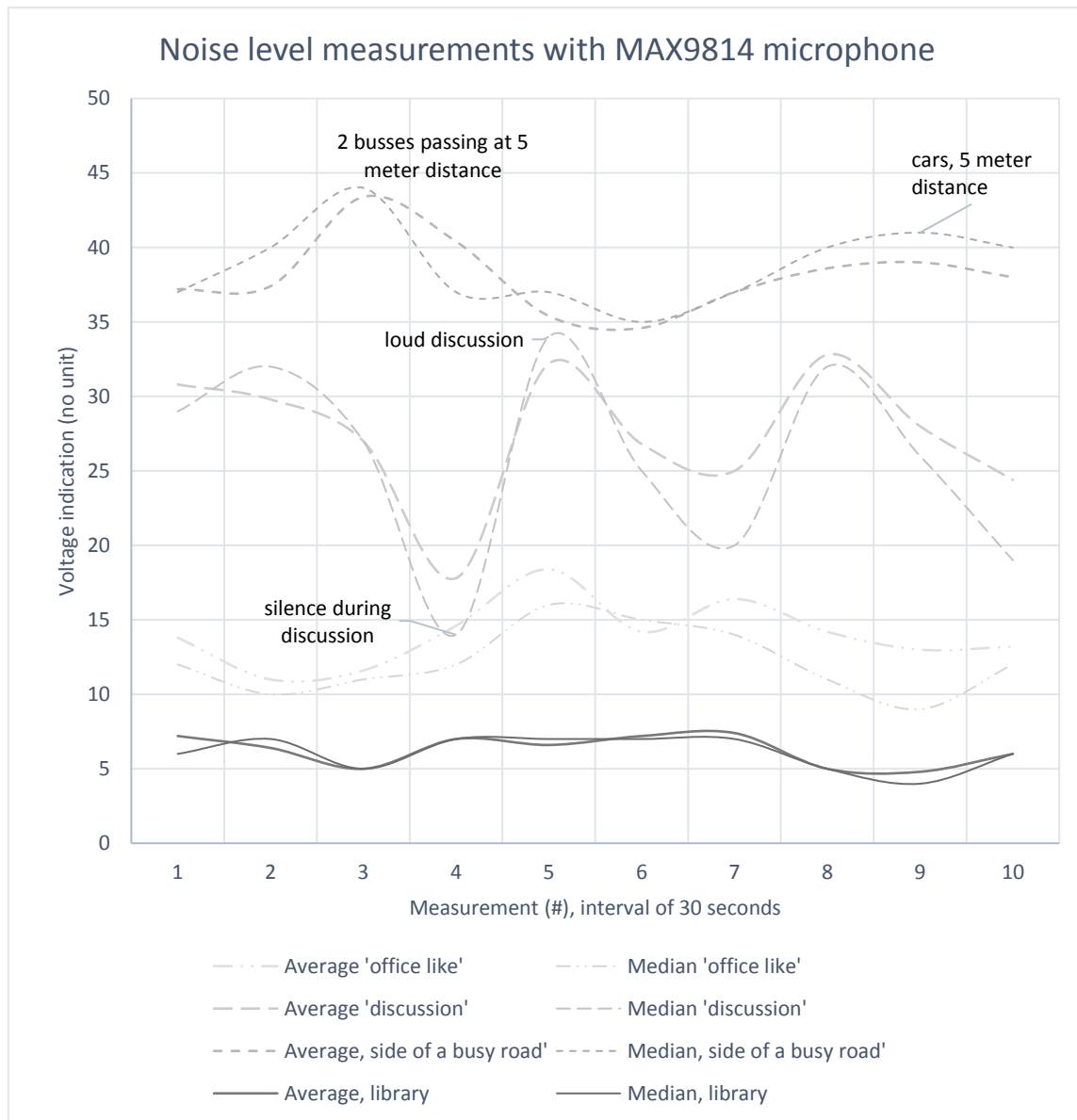
Figure 3: Extra tests with MAX9814 microphone/noise sensor
