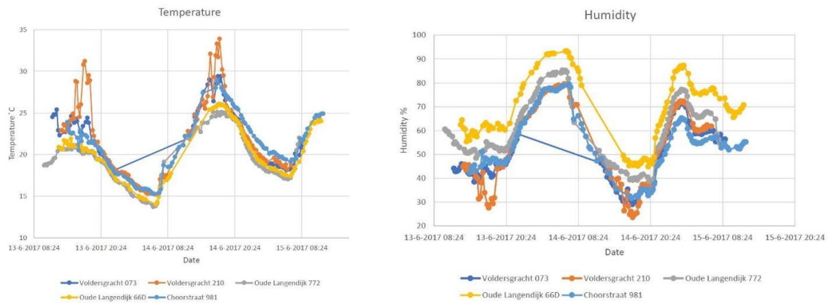
Figure 2: Temperature and humidity measurement results
