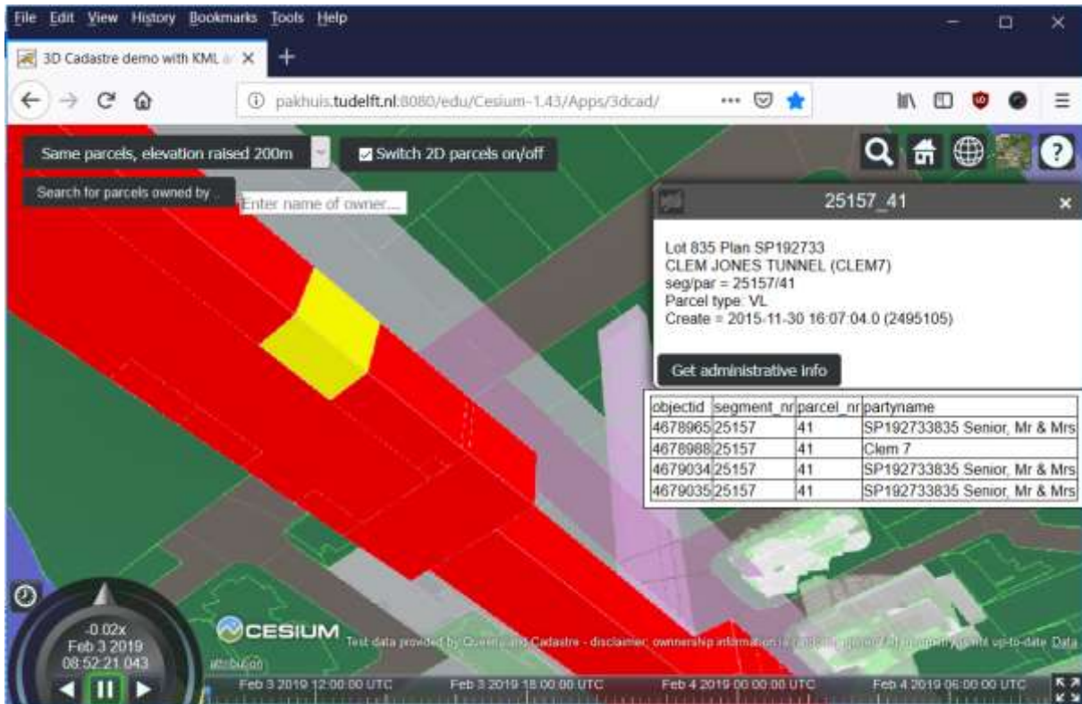
Figure 3. The improved version of the “Get administrative info” now showing all associated records (objectid’s) and their related owners (partyname).
