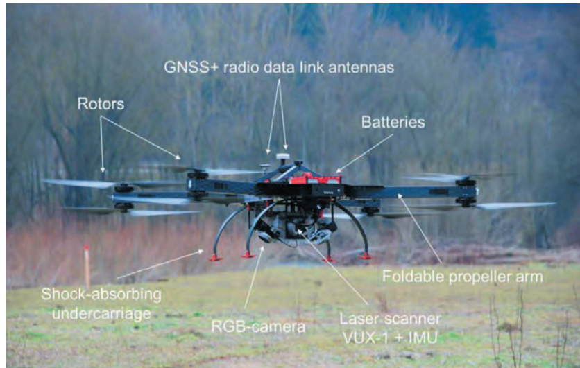
▲ Due to ongoing miniaturization copters are able to carry camera and Lidar sensors simultaneously. (Courtesy: XXX)
