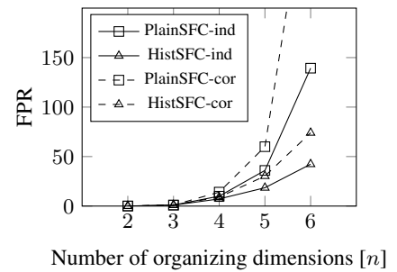
Figure 11. Mean FPR for 2-nD query in RealSim
