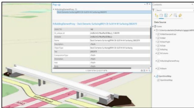
Figure 7. Information about the deck of the bridge model, modelled at the 'LA_LegalSpaceInfrastructure' class.
