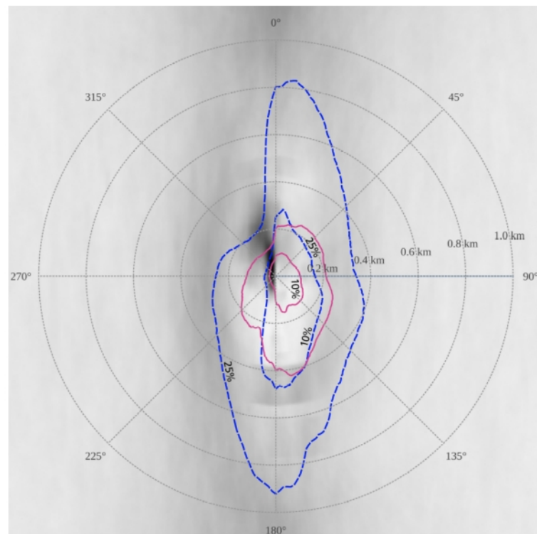
Figure 4: Influence of maximum search radius on the ship domain contours for 10% and 25% usage (maximum search radius for blue: 2.5km, red: 1.0km)
