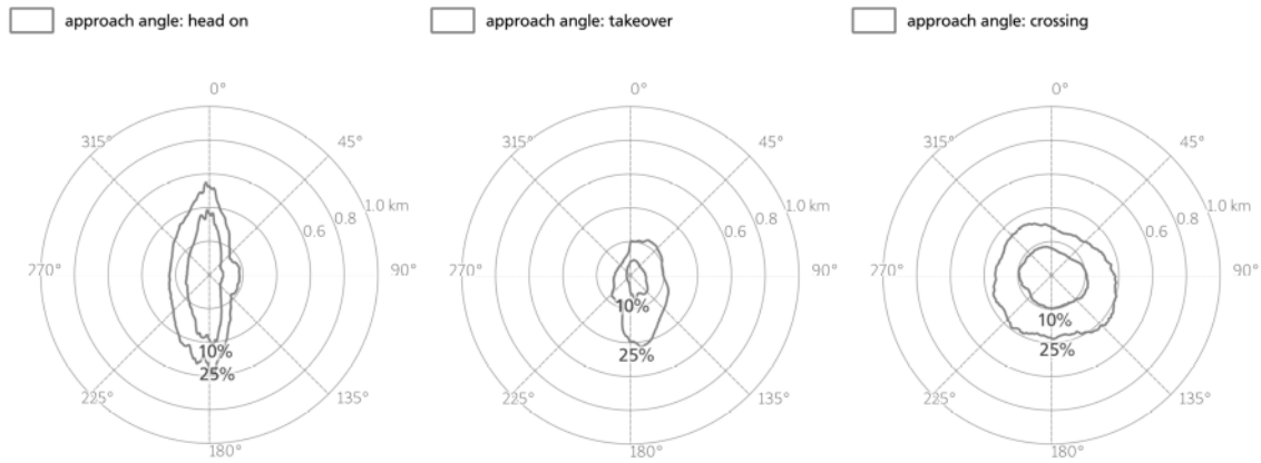
Figure 6: Approach angles: crossing, takeover, head-on ( \Delta\text{COG} ).
