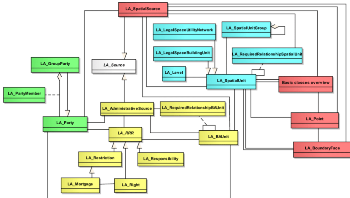
Figure 12. The Land Administration Domain Model. Green: party package, yellow: administrative package, blue: spatial package and red: surveying and representations subpackage (Lemmen et al., 2015).
