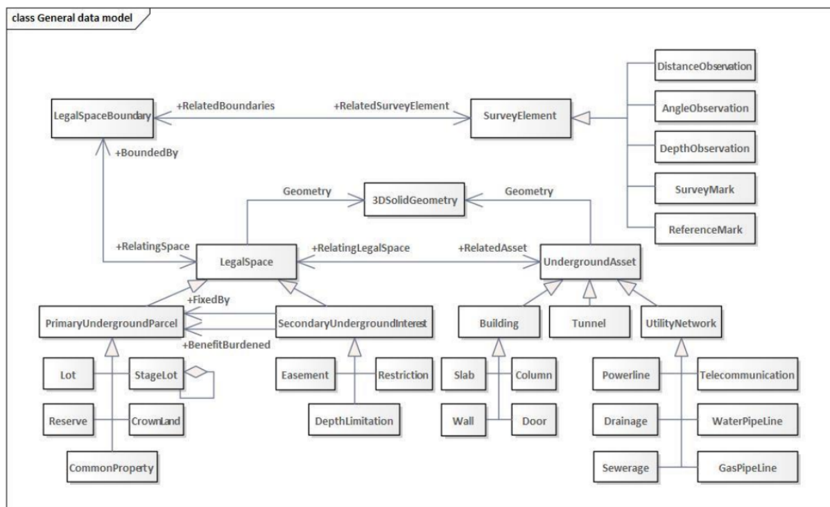
Figure 11. Conceptual data model for underground land administration in Victoria
