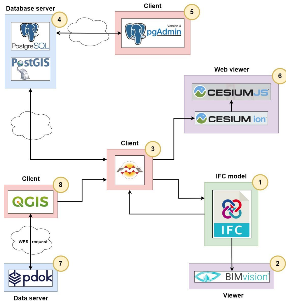
Figure 24. System architecture
