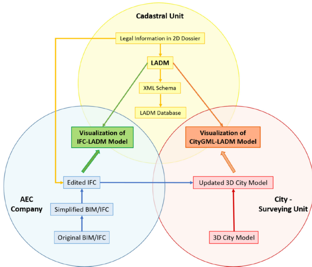
Figure 17. Framework for the combined use of BIM/IFC models with LADM and CityGML (Sun et al., 2019)
