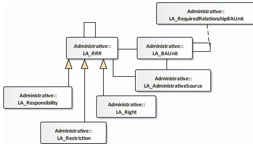
Fig. 8. Classes of Administrative package.
