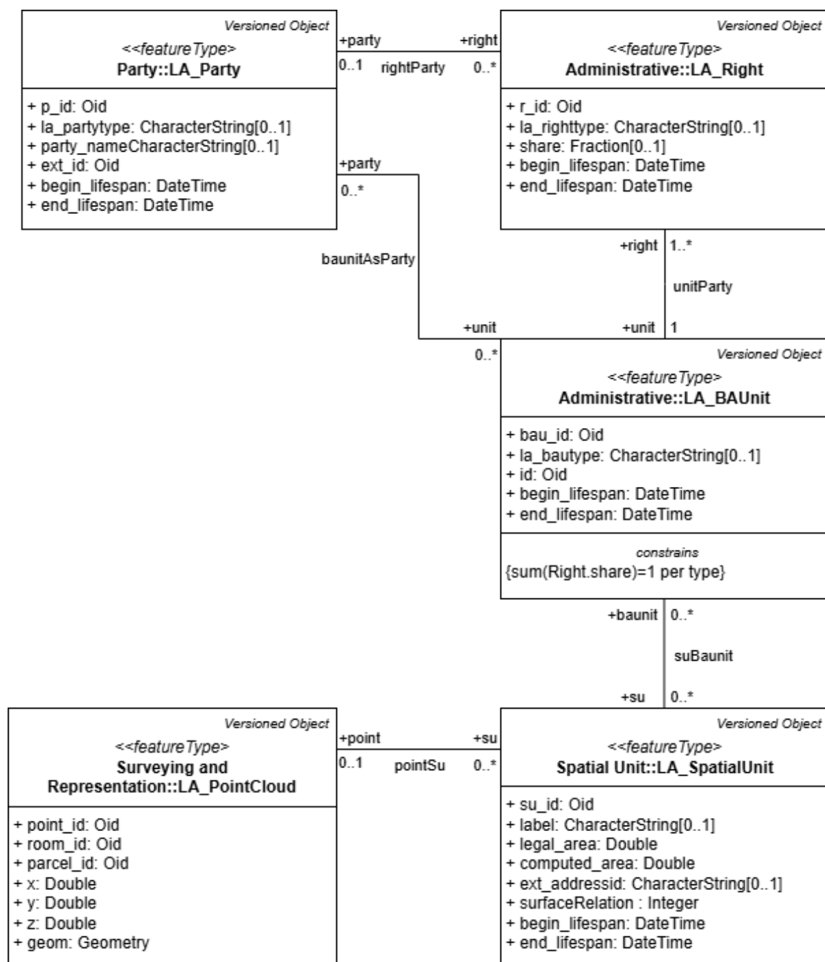
Figure 3. LADM UML Model
