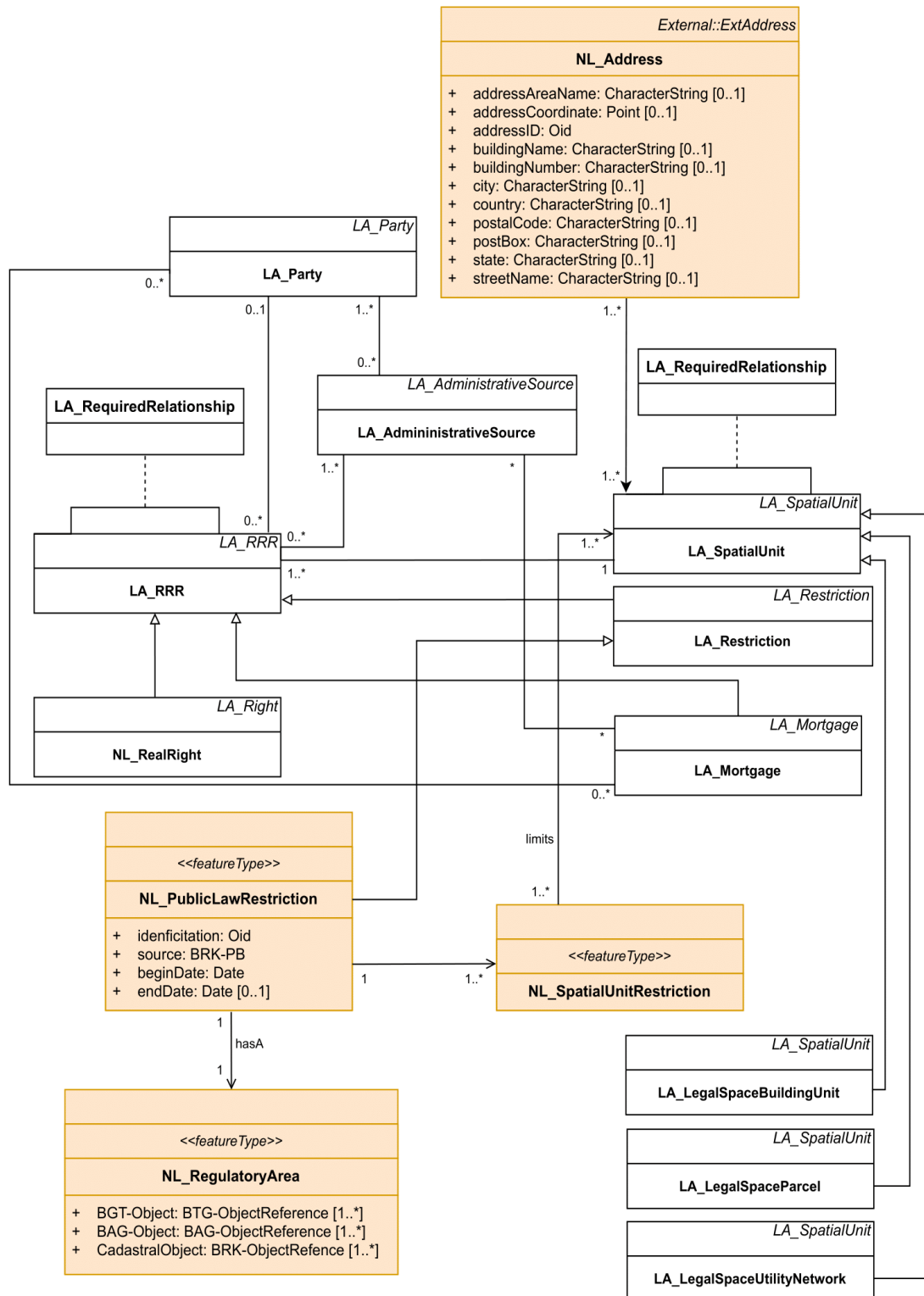
Figure 2. LADM Country profile of the Netherlands for land registry
