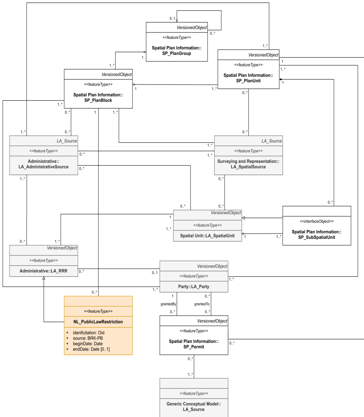
Figure 4. Country profile of the Netherlands for spatial plan information
