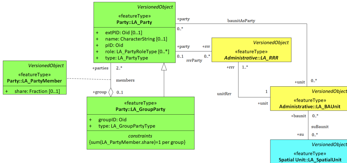
Figure 151. The PartyPackage in green, combined with the core classes LA_RRR (in yellow), LA_BAUnit (in yelow) and LA_SpatialUnit (in blue).
