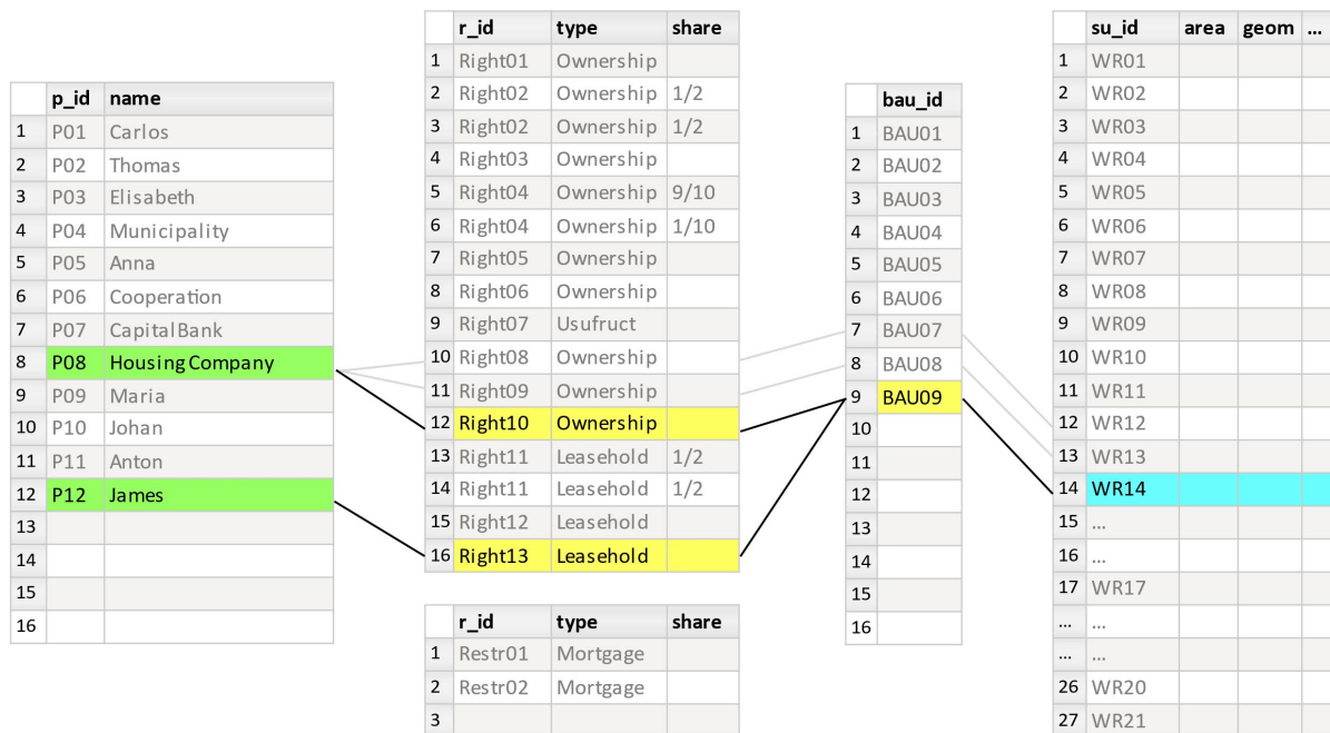
Figure 49. The situation of James in the database.
