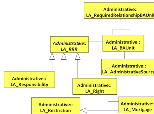
Figure 148. The LADM Administrative Package.
