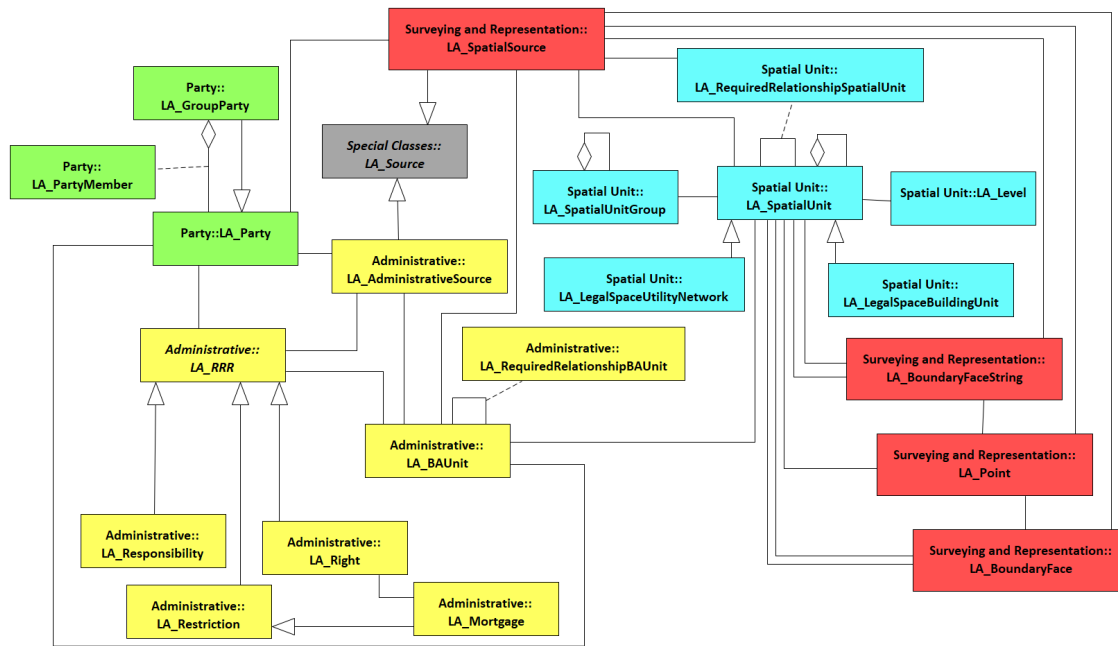
Figure 146. The Land Administration Domain Model: Class Diagram.
