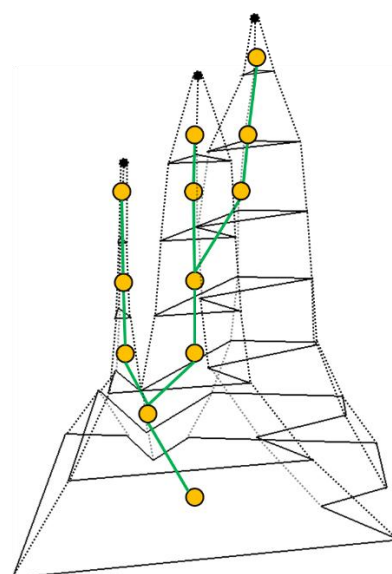
Figure 7. Vario-scale representation and its hierarchical tree structure constructed using the DHE structure. In the primal space, solid black lines represent the spatial geometry (2D and 1D).
